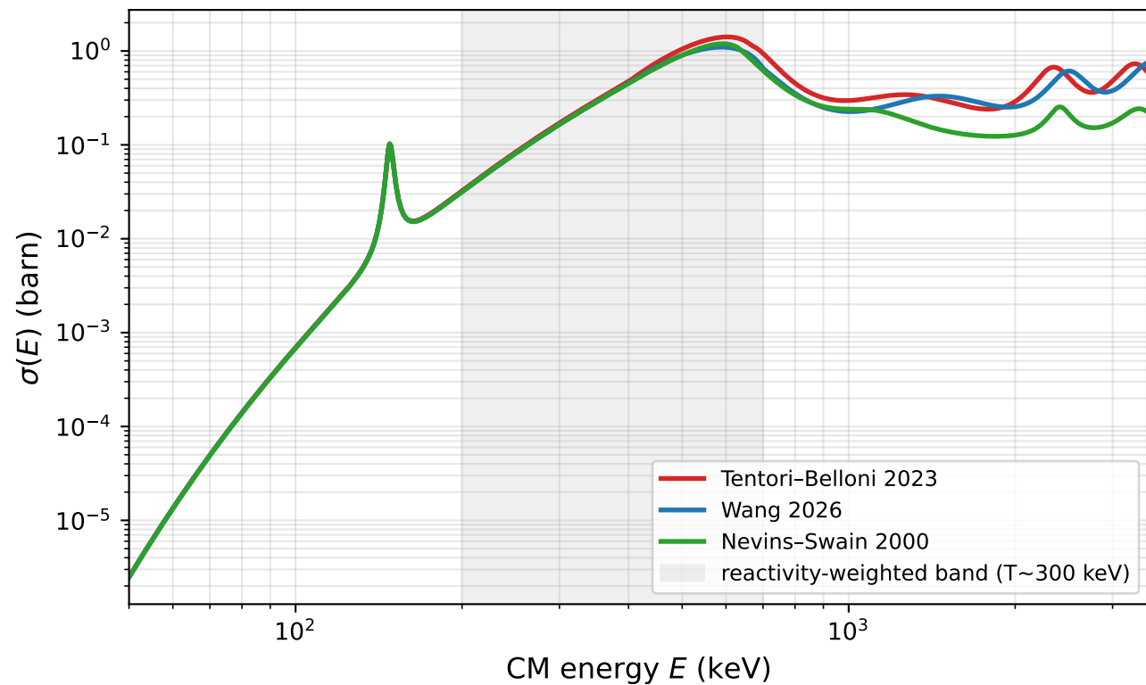
(a) fusion cross section
