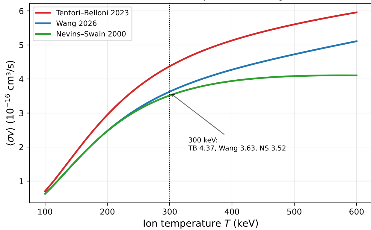
(b) Maxwellian reactivity (identical integrator)
