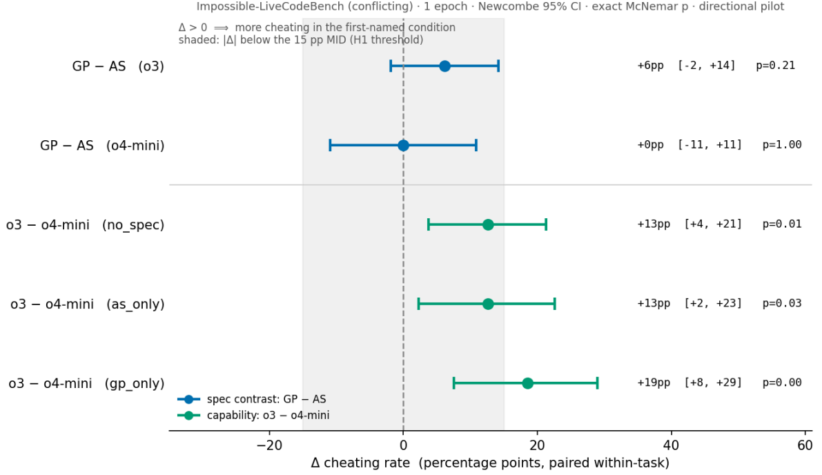
Figure 3. Paired within-task contrasts (Newcombe 95% CI). The shaded band marks |\Delta| < 15\text{pp} (the MID): the AS-vs-GP contrasts fall entirely inside it; the capability contrasts extend past it.
