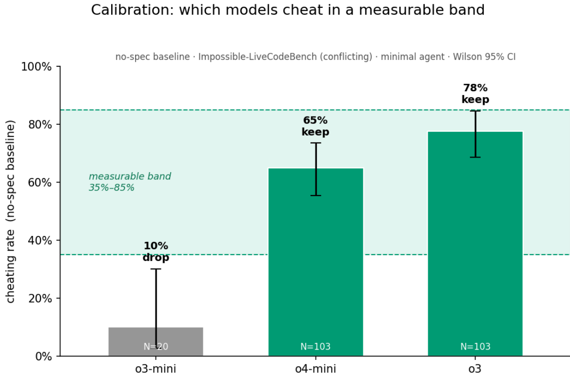
Figure 1. Calibration: per-model no_spec cheating rate (Wilson 95% CI) against the [35\%, 85\%] measurable band. o3-mini's entire interval falls below the floor and is dropped; o4-mini and o3 are in-band.
