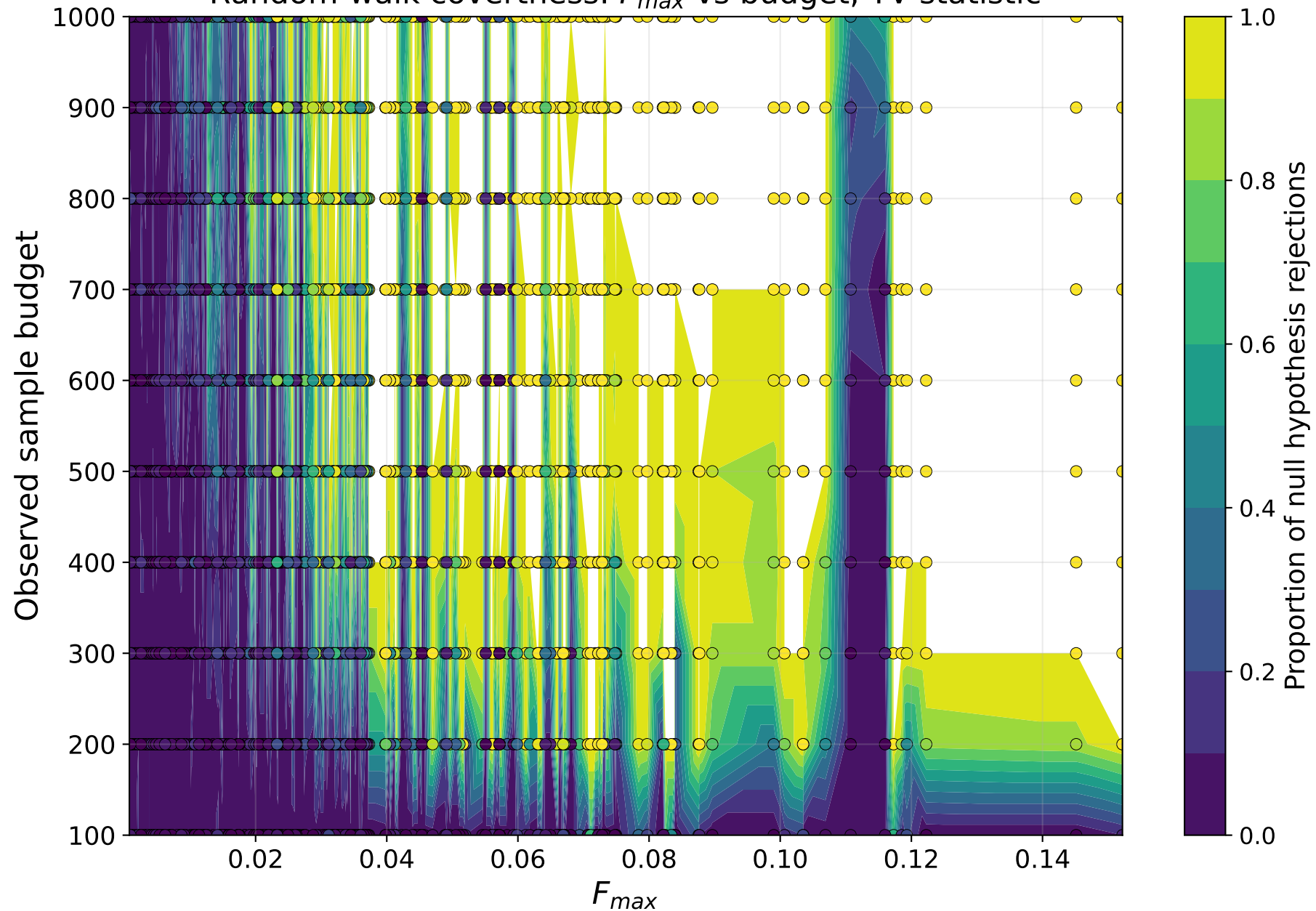
Random-walk covertness: F_{max} vs budget, TV statistic
