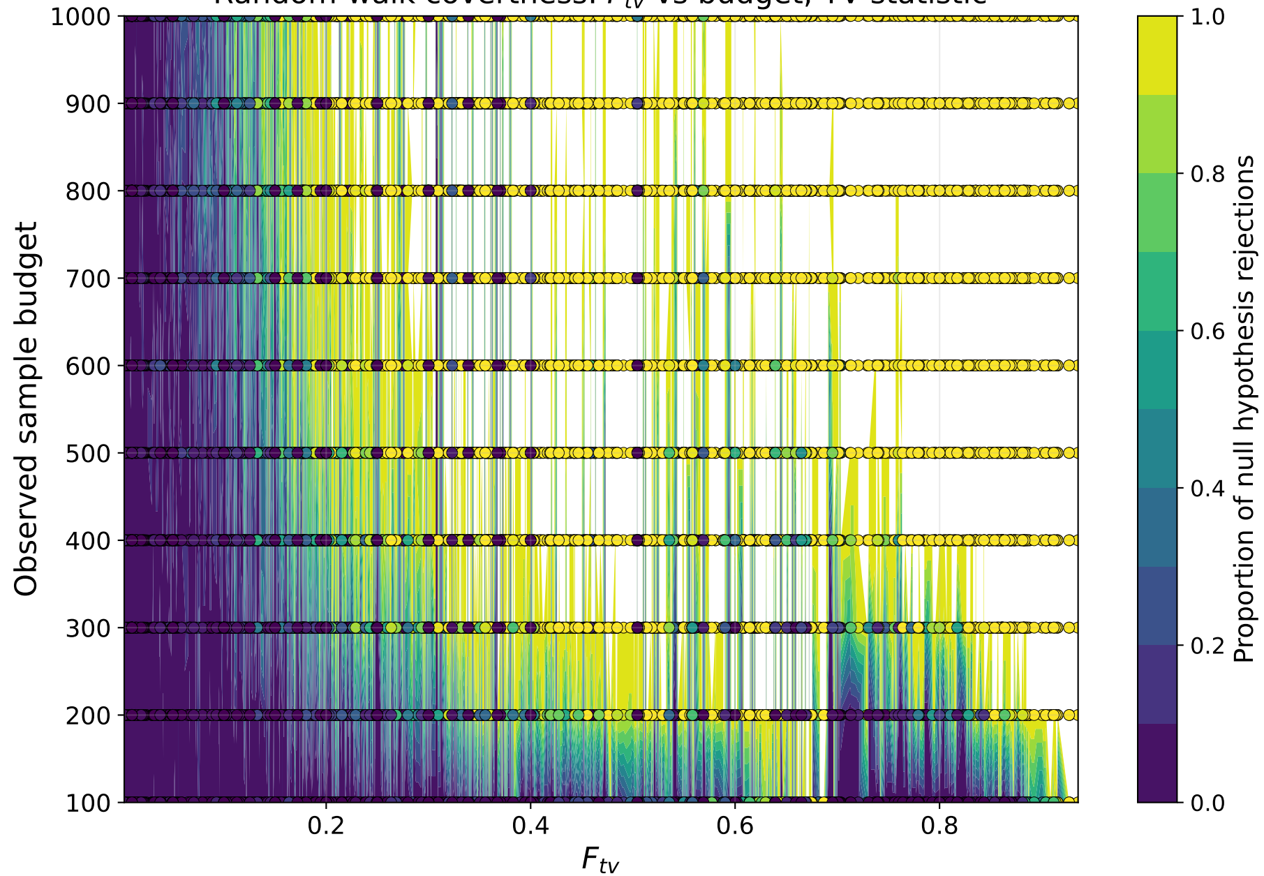
Random-walk covertness: F_{tv} vs budget, TV statistic
