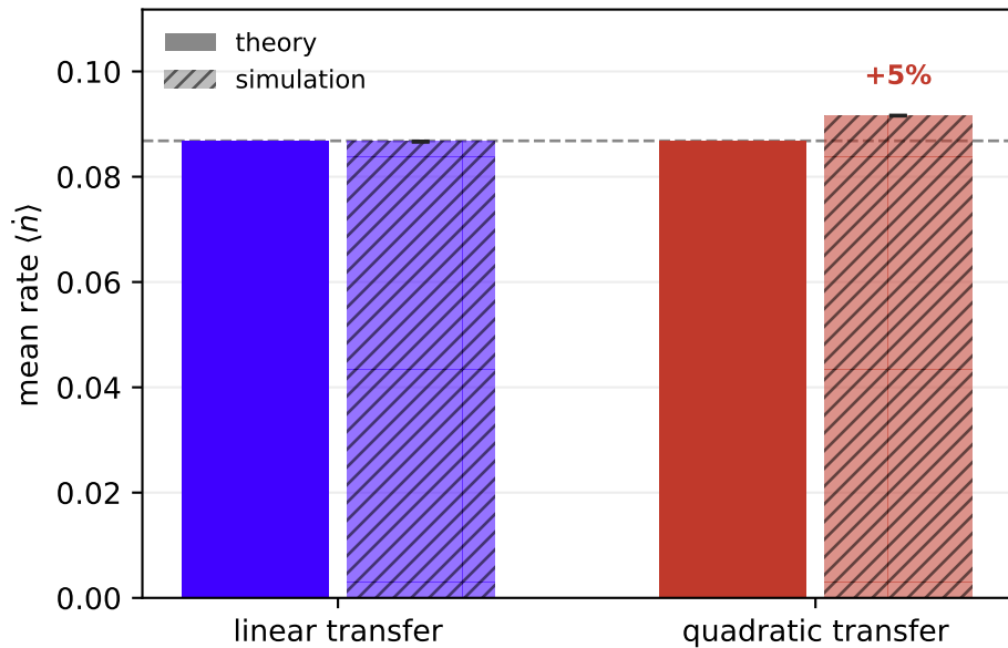
(b) 2-neuron Hawkes: stationary rate
