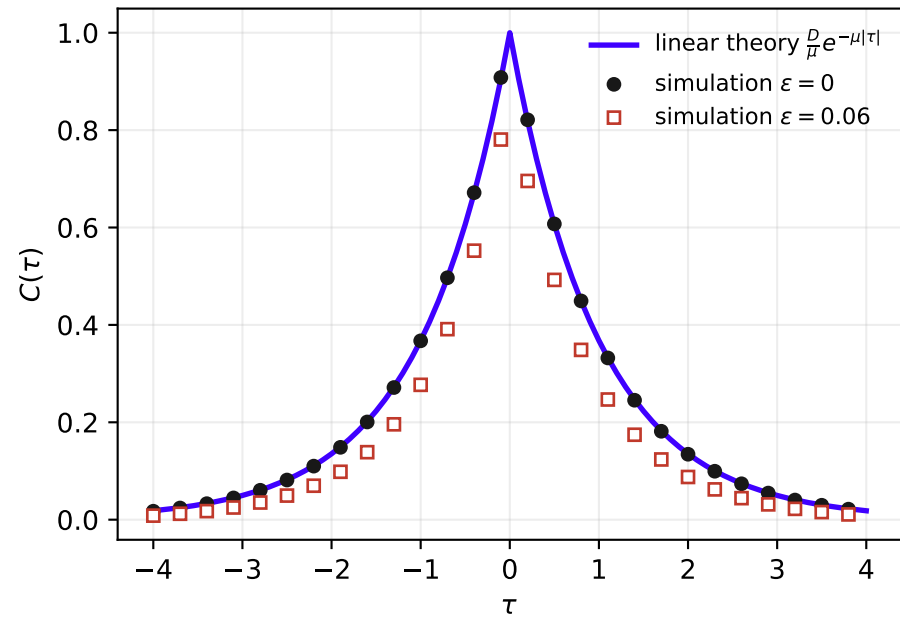
(a) quartic OU: autocovariance
