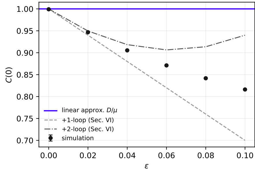
(a) quartic OU: equal-time variance
