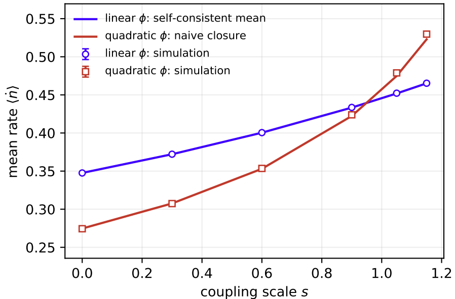
(b) 2-neuron Hawkes: stationary rate
