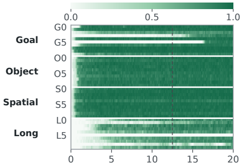
(a) Training SR \tau_k
