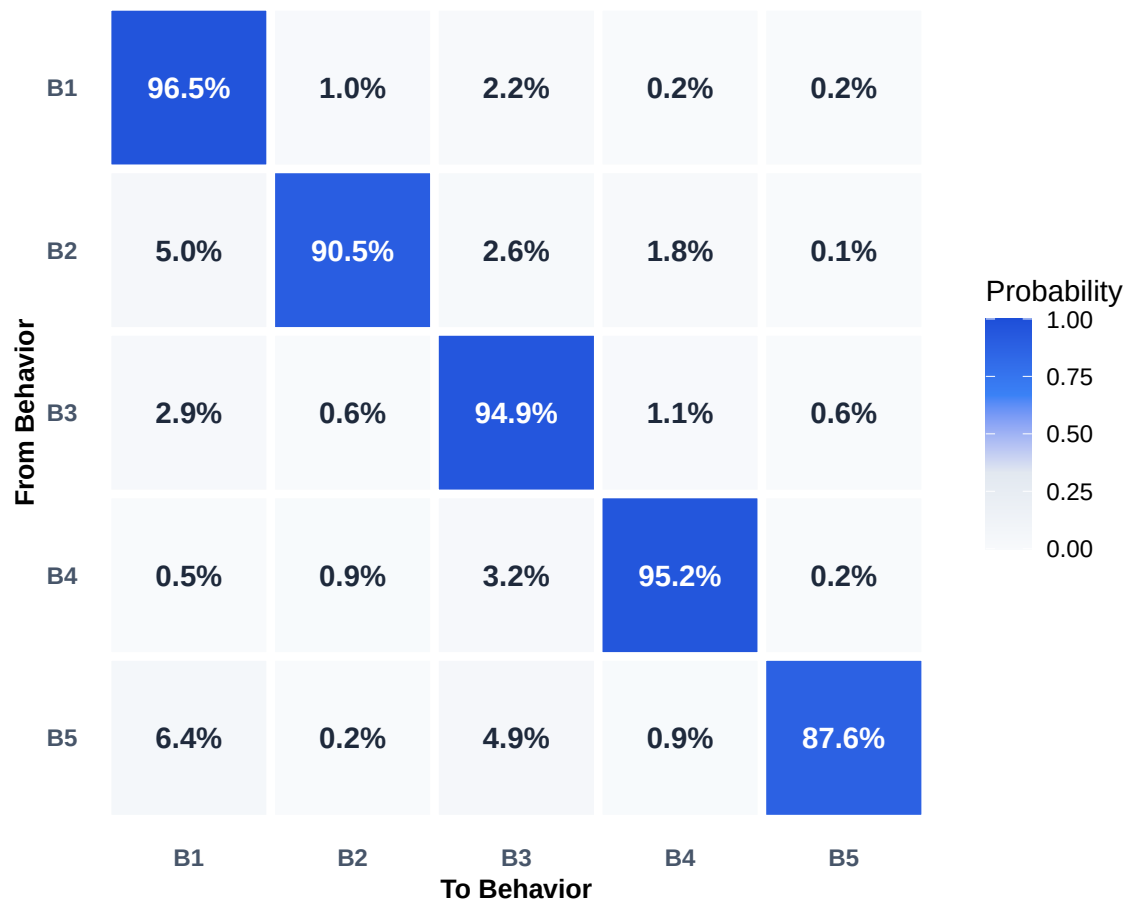
Transition Heatmap: Healthy_Treated
