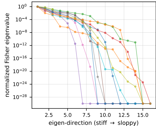
Sloppy spectrum (all conditions)
