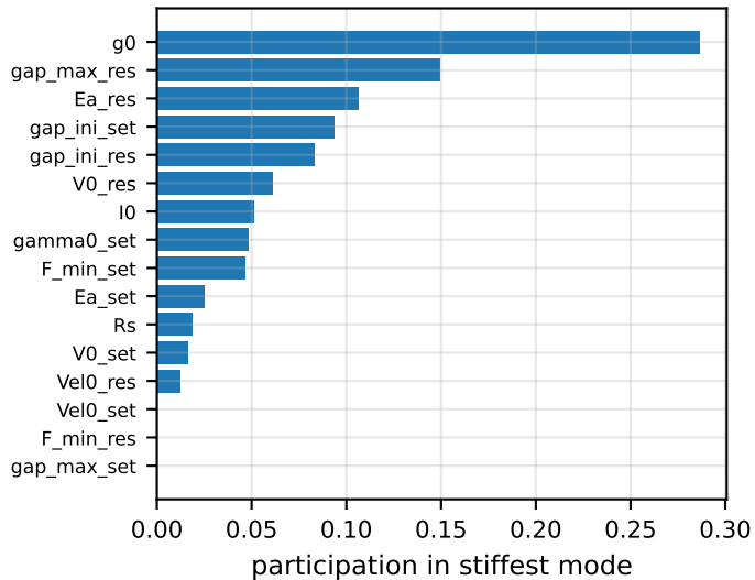
Identifiable direction composition
