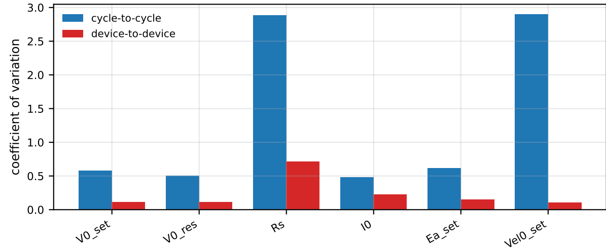
Cycle-to-cycle vs device-to-device spread (center points)
