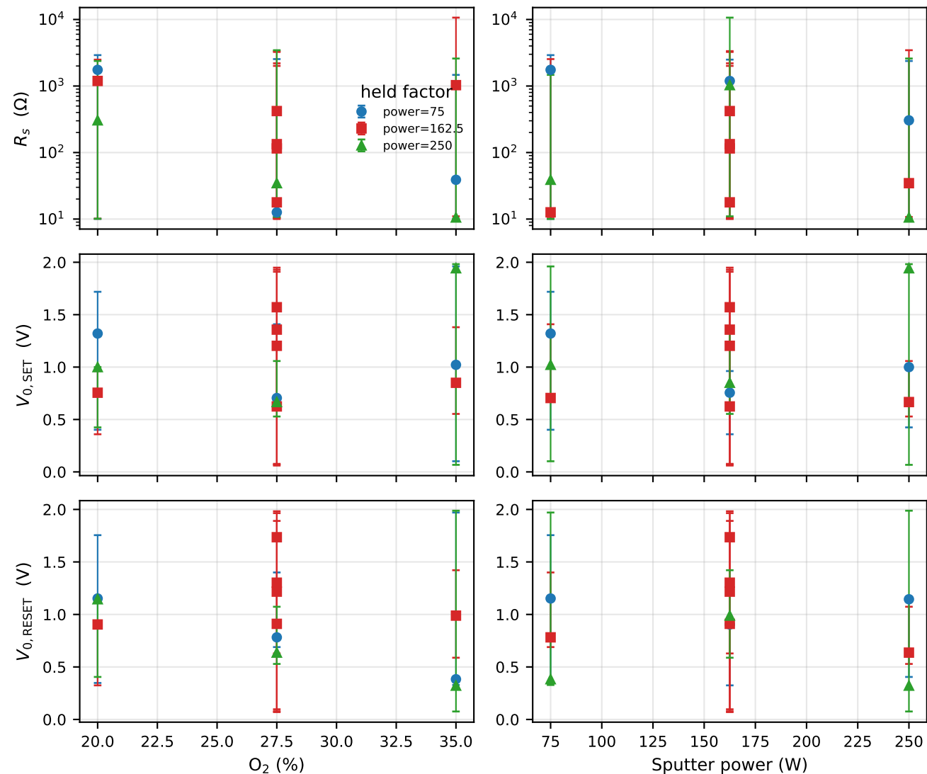
Bootstrap-identifiable parameters vs deposition condition (error bars: cycle-bootstrap 95% CI)
