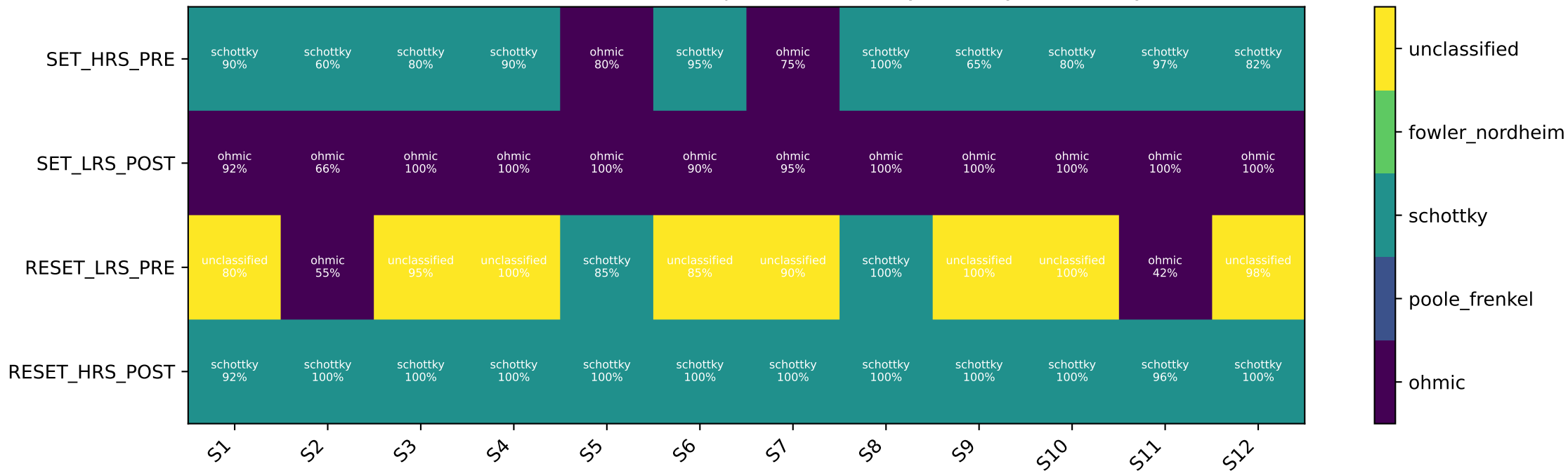
Dominant conduction mechanism per state (% = cycle-to-cycle stability)
