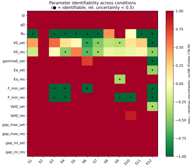
Fig. 5. Fisher relative uncertainty \sigma_\theta/|\theta| (log color scale) for the 16 active Stanford parameters across the twelve conditions; dots mark the nominal identifiable class ( \rho < 0.5 ). The very large condition numbers require these local classifications to be interpreted together with cycle-bootstrap stability.
