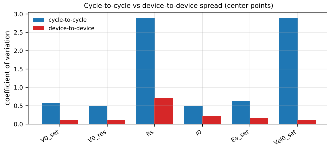
Fig. 7. Cycle-to-cycle versus device-to-device coefficient of variation for representative parameters, from the four replicated center-point devices (S9–S12). Cycle-to-cycle spread dominates for every parameter.
