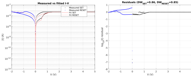
Fig. 3. Measured versus fitted I - V for condition S1 (left) and log-current residuals along the sweep (right). The fit reproduces the butterfly hysteresis, both transitions, and the compliance plateau; the residual concentrates at the SET transition and the Schottky-limited HRS approach.
