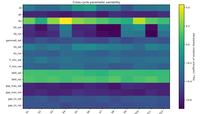
Fig. 6. Cycle-to-cycle parameter variability from 200 cluster-bootstrap refits per condition. Color denotes \log_{10}(\text{CV}) . Series resistance and velocity prefactors are the least stable, while the branch voltage scales are comparatively repeatable.
