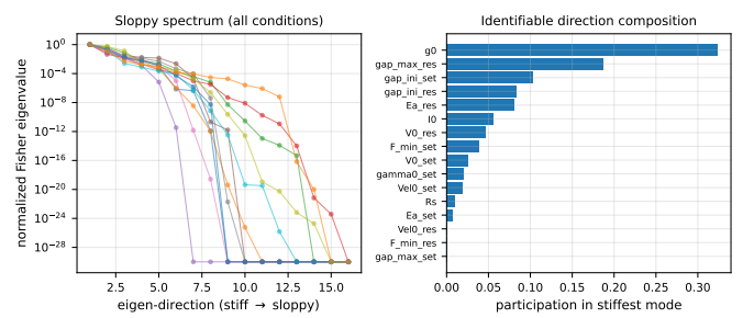
Fig. 4. Sloppiness of the Stanford parameterization. Left: normalized Fisher eigenvalue spectra for all twelve conditions, falling over tens of decades. Right: mean participation of each active parameter in the stiffest (best-determined) eigen-direction—a coupled current-scale/gap combination, not any individual microscopic parameter.
