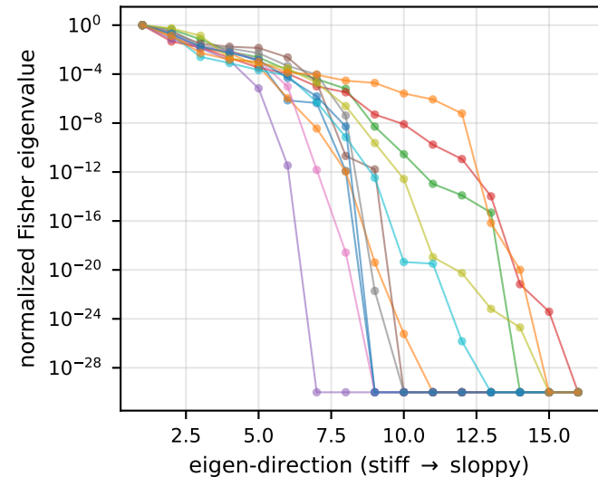
Sloppy spectrum (all conditions)
