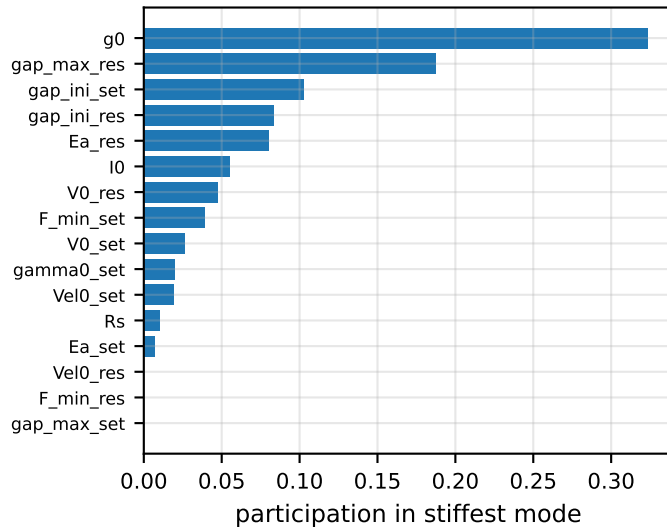
Identifiable direction composition
