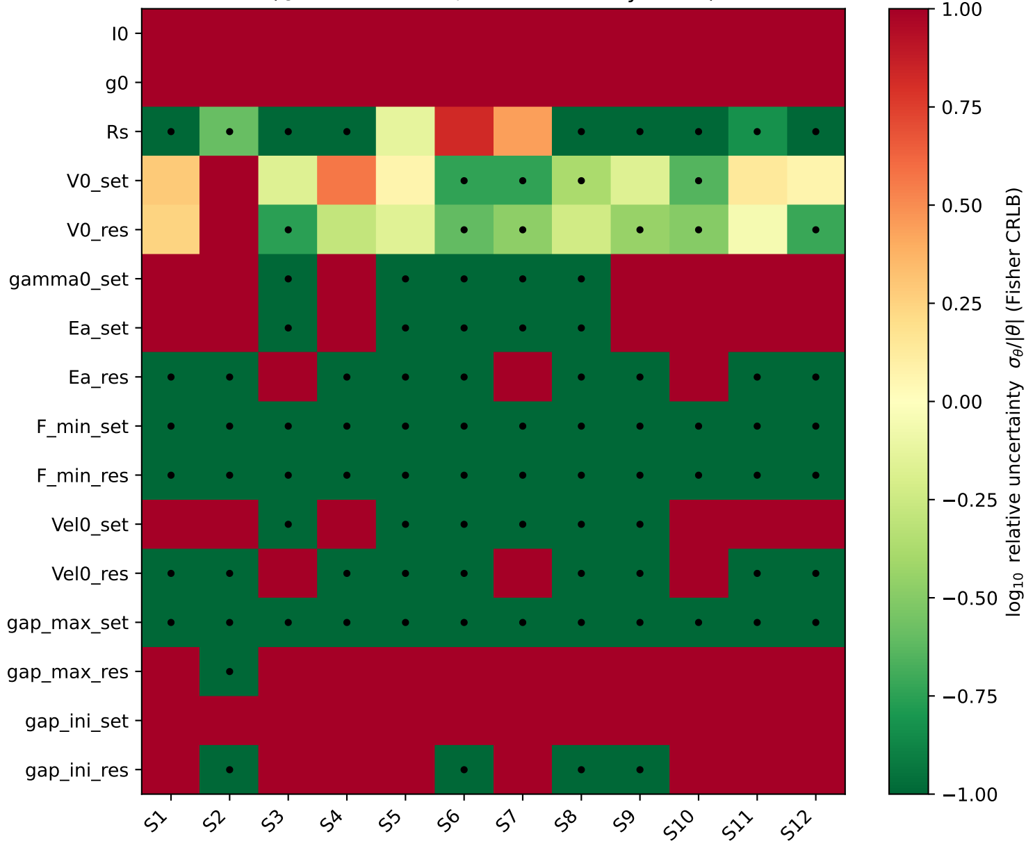
Parameter identifiability across conditions (● = identifiable, rel. uncertainty < 0.5)
