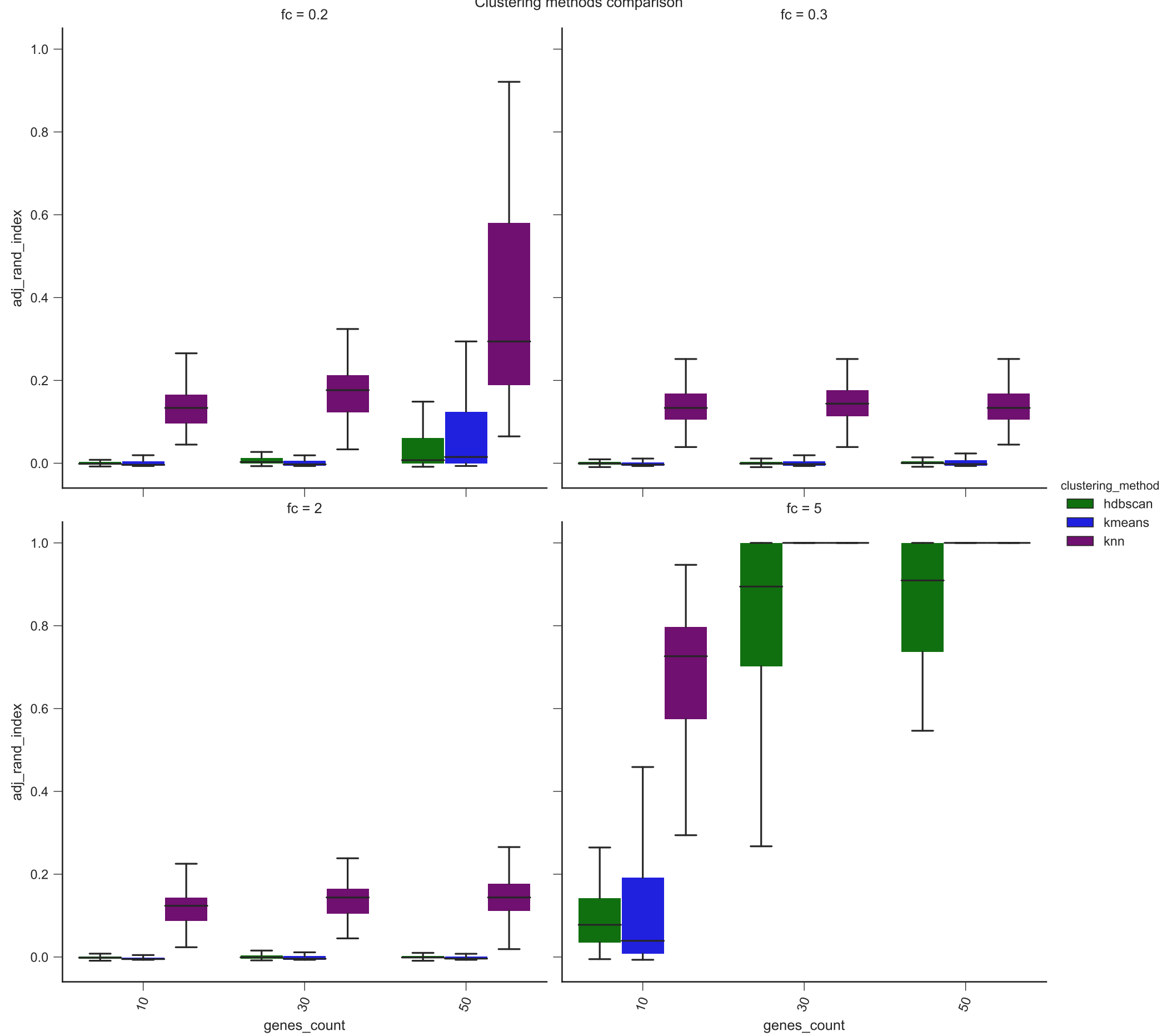
Clustering methods comparison
