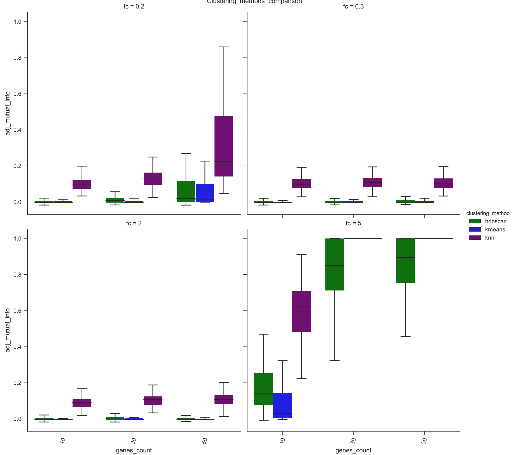
Clustering_methods_comparison
