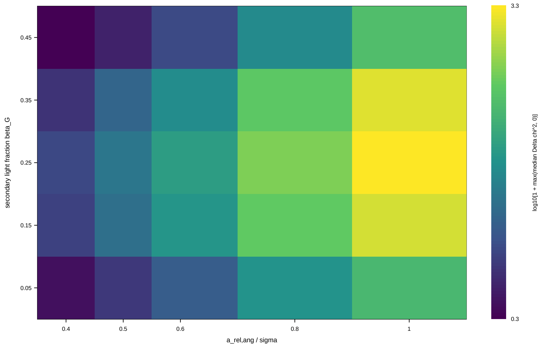
Full-sky single-peak photocentre mismatch
