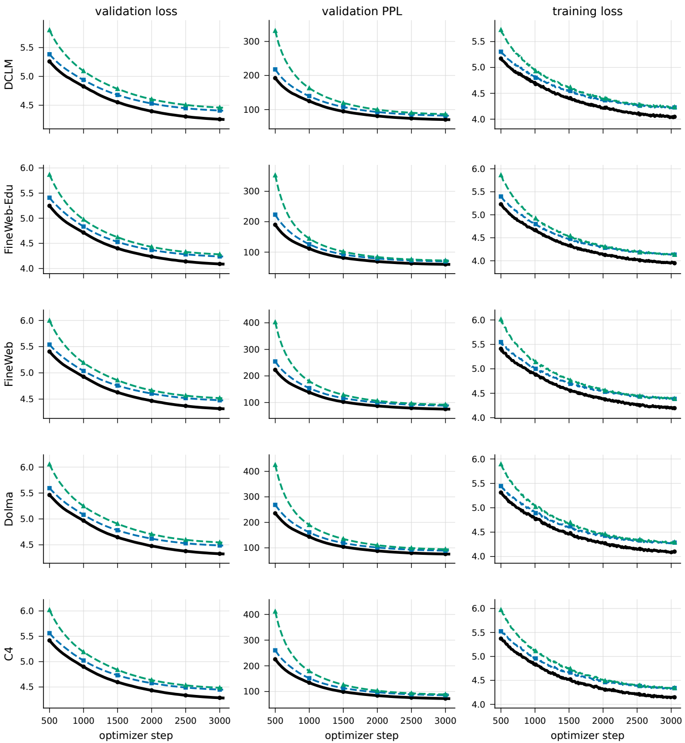
100M-token budget: five datasets by three training metrics
