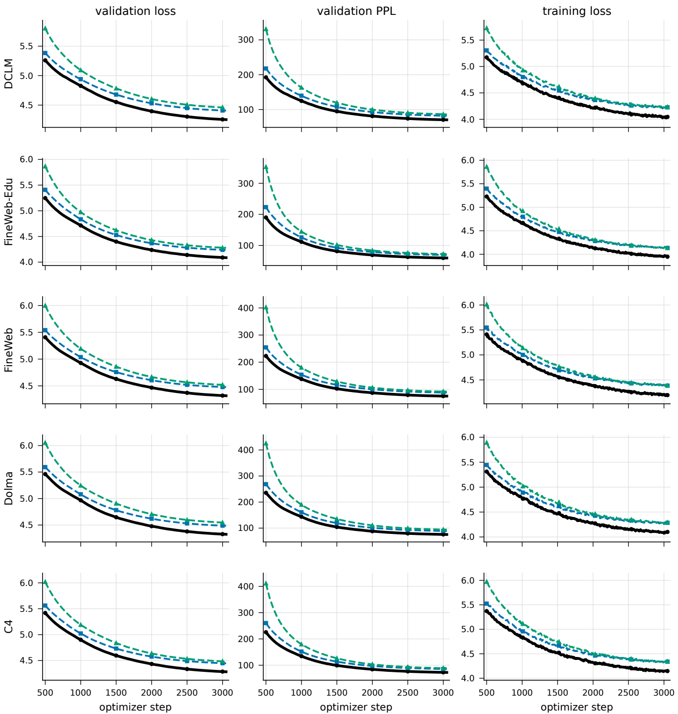
100M-token budget: five datasets by three training metrics
