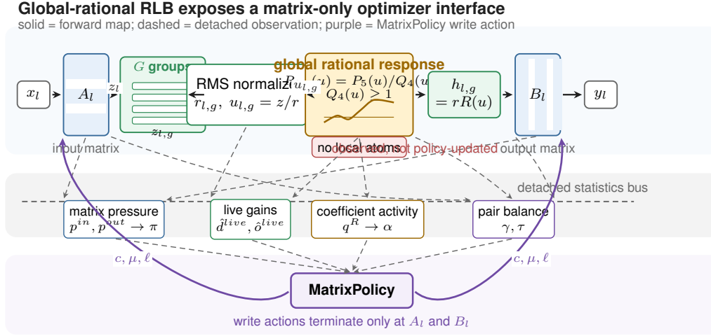
Figure 1: Global-rational RLB exposes an optimizer-visible interface. Solid arrows are the forward map x_l \mapsto y_l ; dashed arrows are detached statistics read by MatrixPolicy; purple arrows are MatrixPolicy actions and terminate only at the RLB input/output matrices. The rational response is AdamW-trained and observed by the policy, but it is not a MatrixPolicy update target in the reported configuration.
