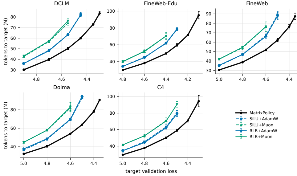
Figure 7: E1 target-arrival frontiers over the pre-specified validation-loss target grid. Lower token counts at the same target indicate faster arrival; vertical bars show one sample standard deviation across three seeds.
