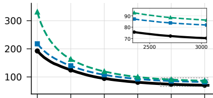
validation perplexity
