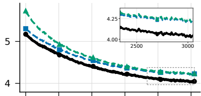
training loss
