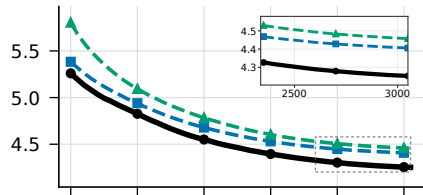
validation loss
