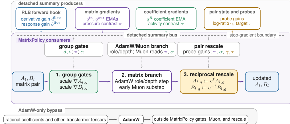
Figure 2: Detached-summary route for the evaluated MatrixPolicy system. The top lane shows where each detached summary family is produced, the middle cards show which MatrixPolicy operation consumes each family, and the bottom lane separates AdamW-only tensors from the matrix-pair update path.
