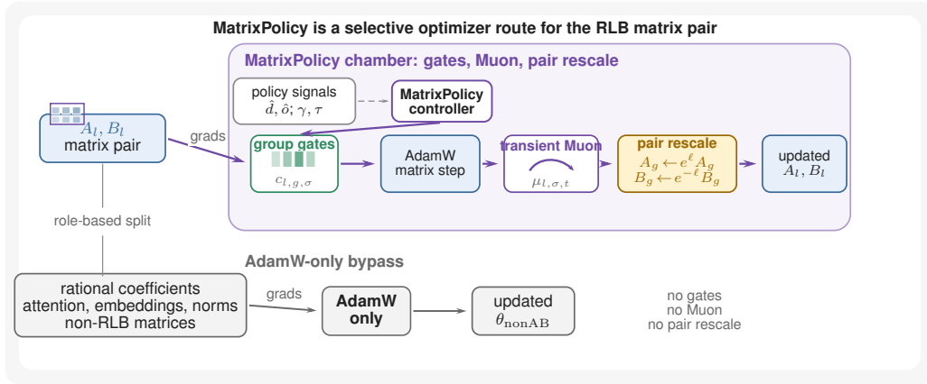
Figure 2: Selective MatrixPolicy route for the reported optimizer. Only the RLB matrix pair A_l, B_l enters the MatrixPolicy chamber: policy signals set group gradient gates c_{l,g,\sigma} , AdamW supplies the base matrix step, a transient Muon correction acts on the same matrices, and pair rescaling applies reciprocal updates A_g \leftarrow e^\ell A_g and B_g \leftarrow e^{-\ell} B_g to move the current balance \gamma toward the target \tau . Rational coefficients and all non-RLB matrix parameters bypass this route and remain AdamW-only.
