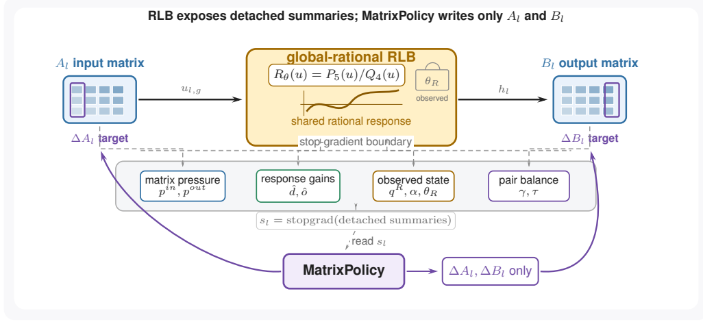
Figure 1: Activation-optimizer interface for global-rational RLB. In layer l , A_l maps the sub-layer input into normalized rational groups and B_l recombines the rational features. RLB exposes matrix-pressure, response-gain, observed-rational-state, and pair-balance summaries through a stop-gradient boundary. MatrixPolicy reads the resulting summary vector s_l and writes only \Delta A_l and \Delta B_l ; rational coefficients are AdamW-trained and policy-observed, not MatrixPolicy update targets.
