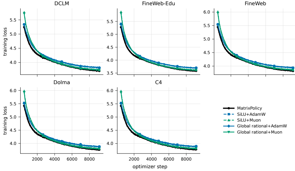
Figure 10: 300M-token-budget training-loss trajectories for the same comparator set.
