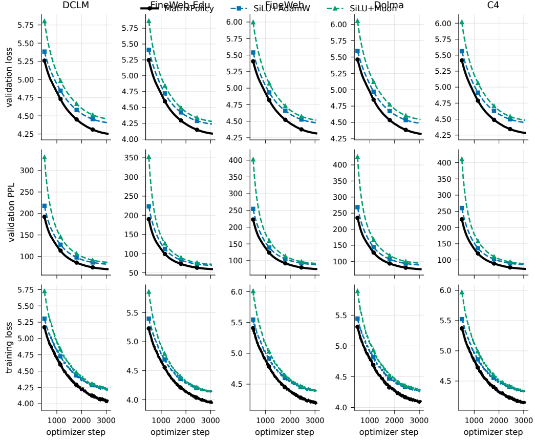
Figure 6: Full 100M-token-budget multi-metric trajectories across all five datasets for the main SiLU comparison. Rows show validation loss, validation perplexity, and training loss; columns show datasets. Lines are seed means and bands show one sample standard deviation.
