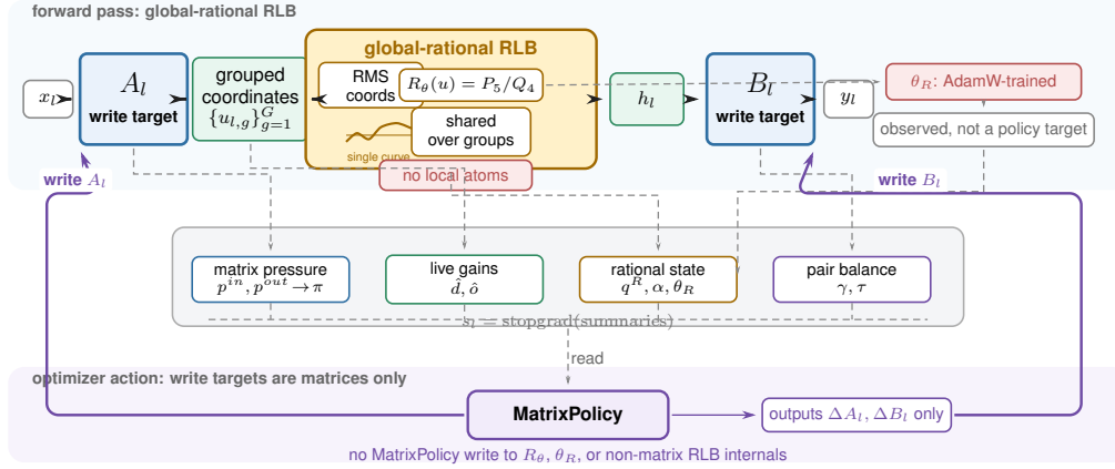
Figure 1: Global-rational RLB exposes an optimizer-visible interface. Solid arrows are the forward map x_l \mapsto y_l ; dashed arrows are detached statistics read by MatrixPolicy; purple arrows are MatrixPolicy actions and terminate only at the RLB input/output matrices. The rational response is AdamW-trained and observed by the policy, but it is not a MatrixPolicy update target in the reported configuration.
