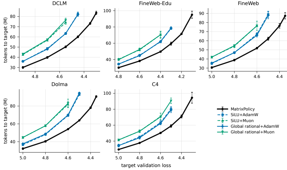
Figure 7: 100M-token-budget target-arrival frontiers over the pre-specified validation-loss target grid. Lower token counts at the same target indicate faster arrival; vertical bars show one sample standard deviation across three seeds.
