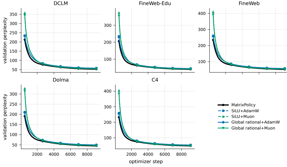
Figure 9: 300M-token-budget validation-perplexity trajectories for the same comparator set.
