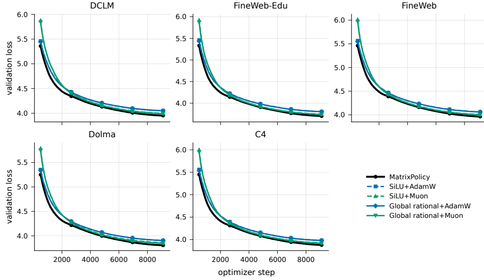
Figure 8: 300M-token-budget validation-loss trajectories for the same comparator set used in the appendix 100M-token-budget control figures. These longer-budget curves support the saturation discussion in Section 4.
