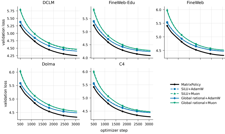
Figure 5: 100M-token-budget validation-loss trajectories for MatrixPolicy, SiLU baselines, and RLB optimizer controls. Lines are seed means and bands show one sample standard deviation.
