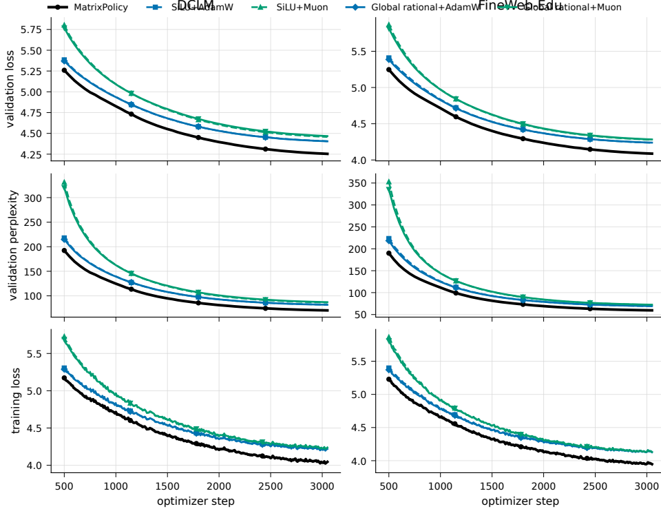
Figure 11: Representative 100M-token-budget validation-perplexity and training-loss companions on DCLM and FineWeb-Edu, including the appendix RLB optimizer controls. The main text keeps the corresponding SiLU comparison in Figure 4.
