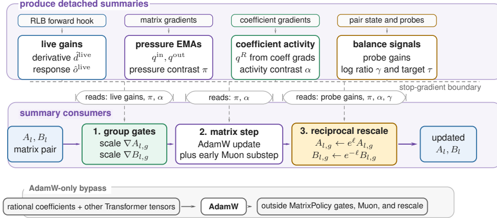
Figure 2: Detached-summary route for the evaluated MatrixPolicy system. The top lane shows where each detached summary family is produced; the middle lane shows where those summaries enter group-gradient gates, the AdamW/Muon matrix branch, and the post-step reciprocal pair rescale. Rational coefficients and non-RLB Transformer parameters remain AdamW-only.
