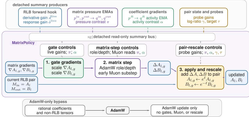
Figure 2: Detached-summary route for the evaluated MatrixPolicy system. The top band produces stop-gradient summaries from forward hooks, pre-policy gradients, and pair probes; the read-only bus routes them to three MatrixPolicy consumers. The lower policy band separates the gradient/update lane from the current matrix-pair state lane, while rational coefficients and non-RLB tensors remain AdamW-only.
