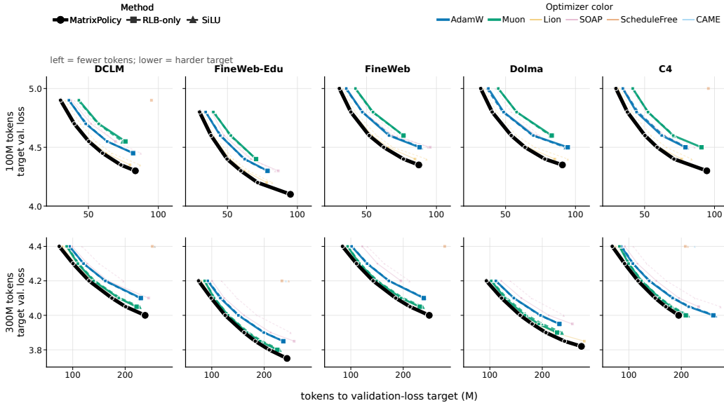
Figure 3: Target-arrival map for the completed fixed-scale study. Rows show the 100M- and 300M-token budgets, and columns show datasets. Each point is the mean token count needed by one method to reach one validation-loss target; connected points trace the same method from easier to harder targets within that dataset-setting panel. The horizontal coordinate is target-arrival tokens, and the vertical coordinate is target validation loss, so curves further left reach the same loss with fewer tokens. The hard-target timing and token-saving percentages are quantified in Table 1.
