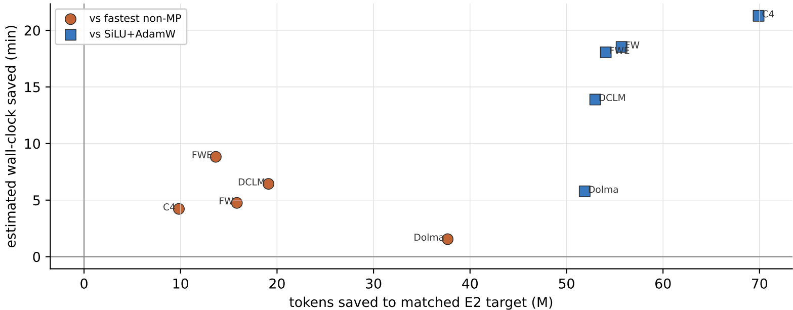
E2 target arrival: fewer tokens and less training time
