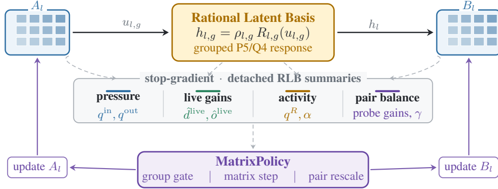
Figure 1: RLB activation-optimizer interface. The matrix A_l forms normalized rational groups and B_l recombines h_l = \text{concat}_{g=1}^G h_{l,g} . Detached forward, gradient, coefficient-activity, and pair-balance summaries condition MatrixPolicy updates of (A_l, B_l) ; rational coefficients follow AdamW.
