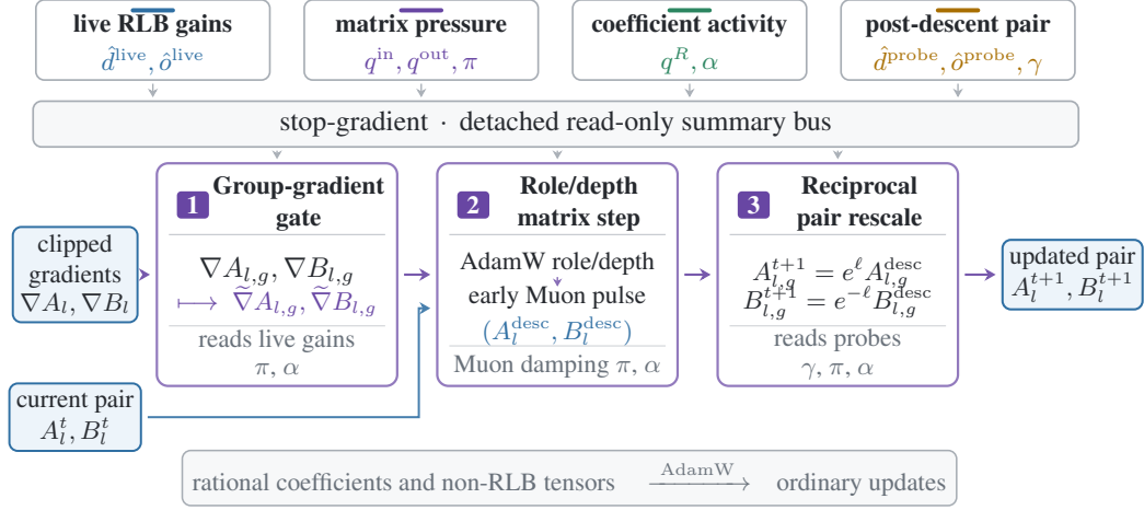
Figure 2: MatrixPolicy signal flow. A read-only stop-gradient bus carries forward, gradient, curve-probe, and post-descent pair summaries to the three controls. Separate lower lanes track the gradient update and current pair; rational coefficients and non-RLB tensors follow AdamW.
