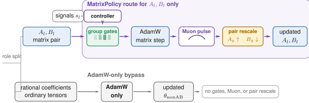
Figure 2: Selective MatrixPolicy route for the reported optimizer. Only the RLB matrix pair A_l, B_l enters the MatrixPolicy chamber: policy signals set group gradient gates c_{l,g,\sigma} , AdamW supplies the base matrix step, a transient Muon correction acts on the same matrices, and pair rescaling applies reciprocal updates A_g \leftarrow e^\ell A_g and B_g \leftarrow e^{-\ell} B_g to move the current balance \gamma toward the target \tau . Rational coefficients and all non-RLB matrix parameters bypass this route and remain AdamW-only.
