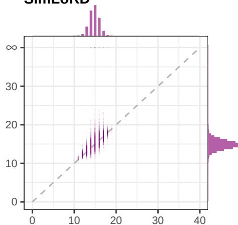
SimLoRD
