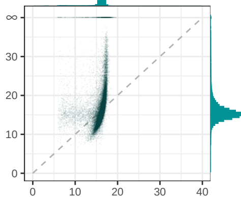
SimLoRD
