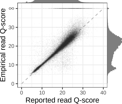
Real reads
