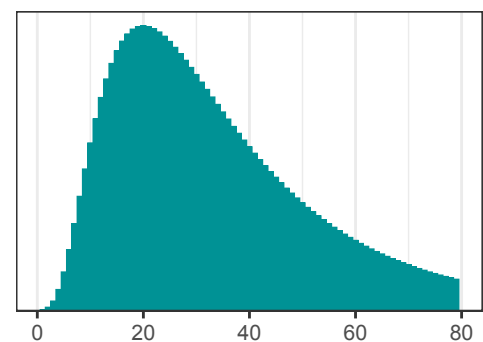
NanoSim
