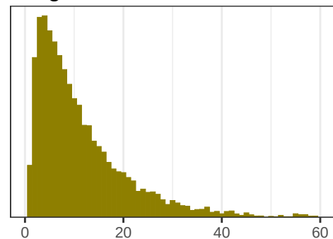
LongISLND
