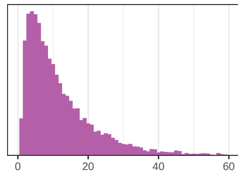
SimLoRD
