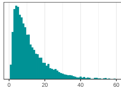
NanoSim
