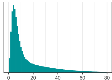
NanoSim
