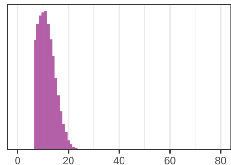
SimLoRD
