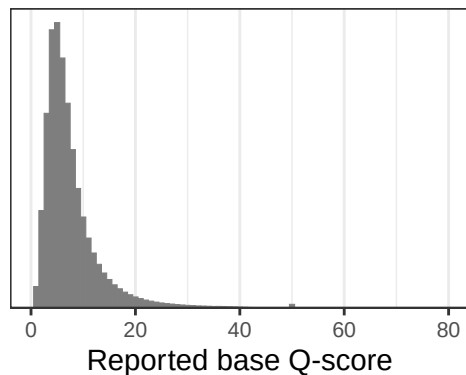
Real reads
