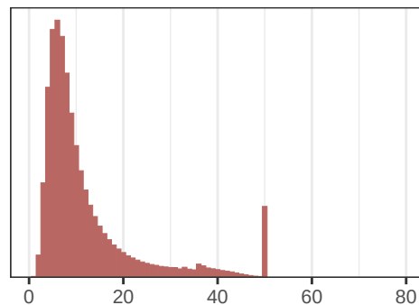
Badread
