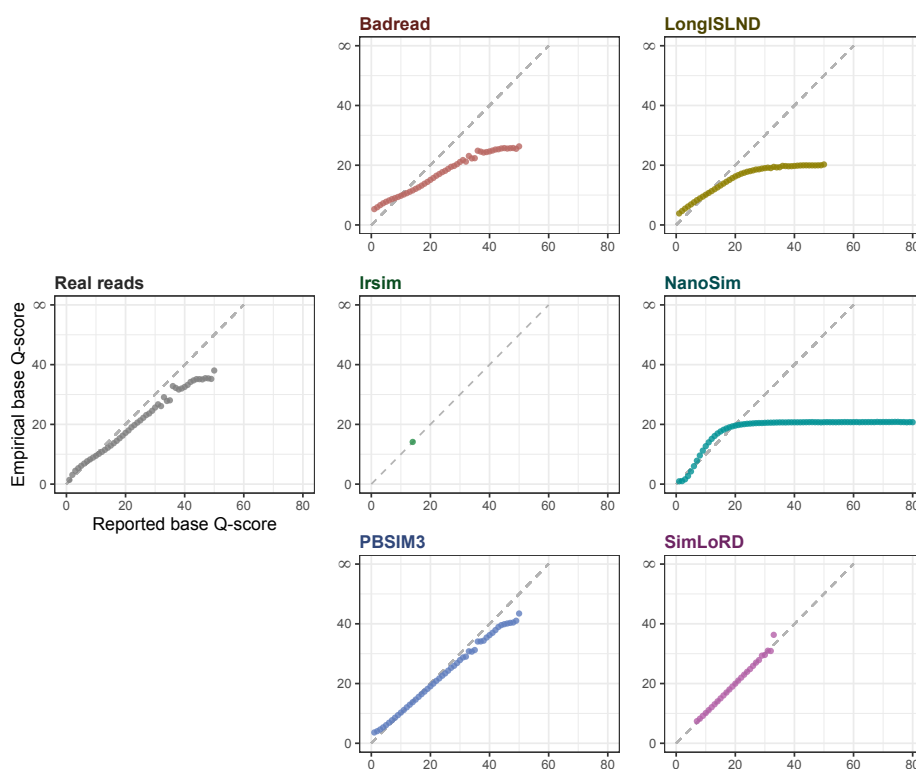
Figure S6: Q-score calibration curve. Per-base Q-score calibration for real and simulated datasets. Each point represents one reported base Q-score bin (x-axis), and its y-value is the empirical base Q-score calculated from the observed error rate among bases with that reported Q-score. Empirical error rate was defined as the fraction of bases in the bin that were mismatches or insertions, plus deletion-associated events estimated as half the count of matched bases adjacent to deletions. The dashed diagonal indicates perfect calibration, where reported and empirical base Q-scores are equal.
