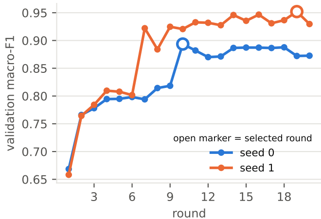
Phase 2: HetGNN
