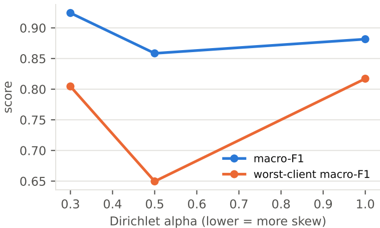
Label skew (E5)
