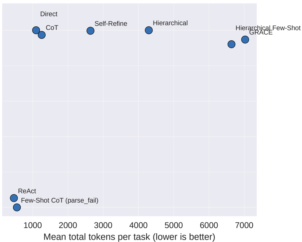
model = mistral-nemo
