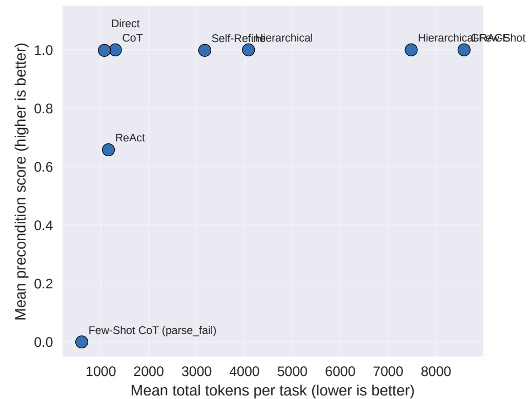
model = llama3.2
