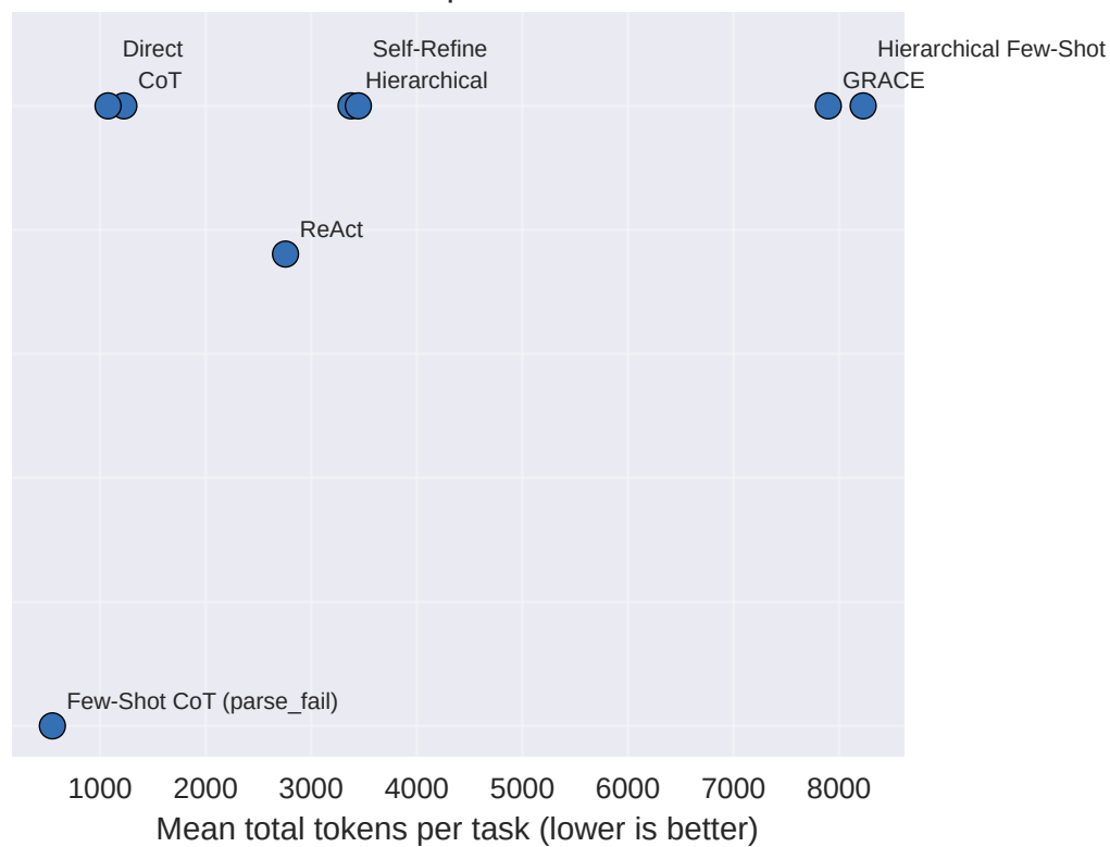
model = qwen2.5:7b
