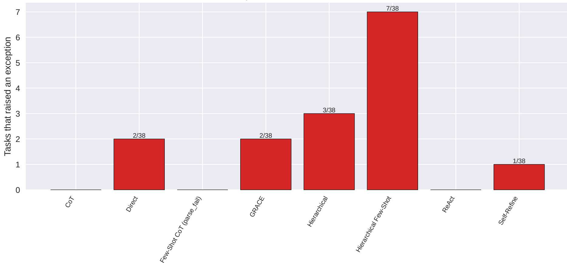
Errors per method — model=llama3.2
