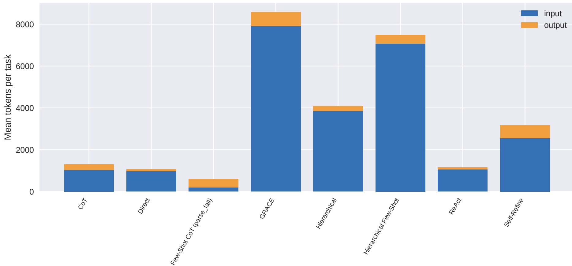
Token breakdown — model=llama3.2
