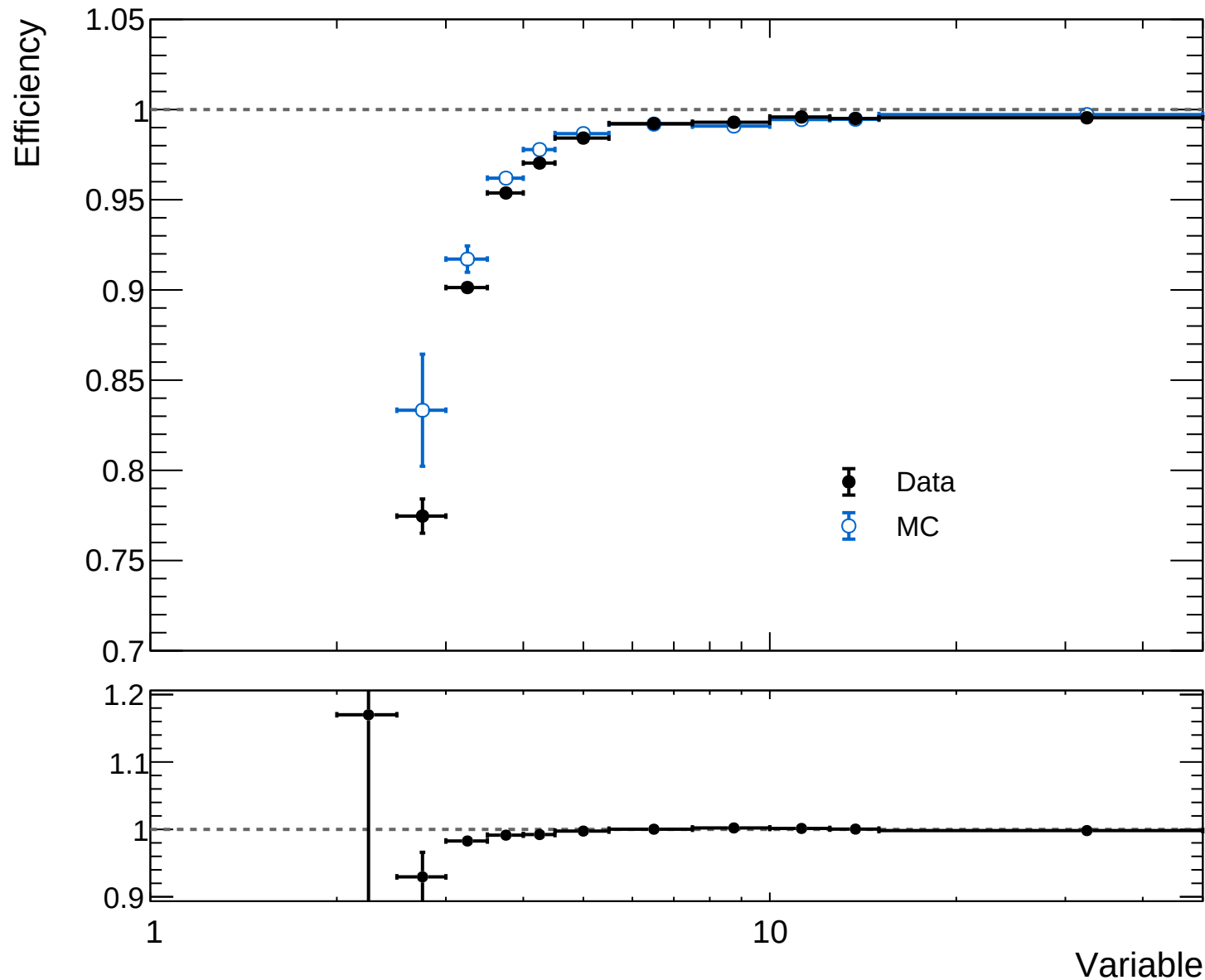
mu_ID: Data vs MC
