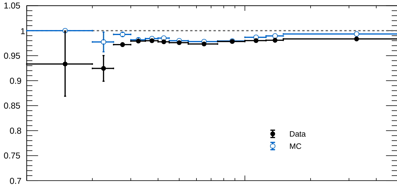
ID_MS: Data vs MC
