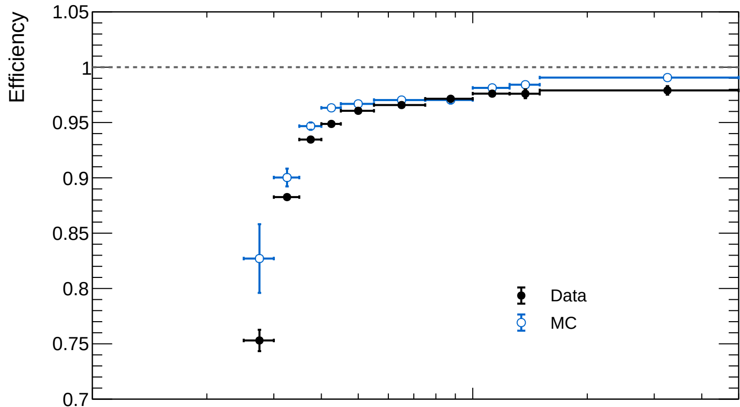
Product (ID_MS x mu_ID): Data vs MC
