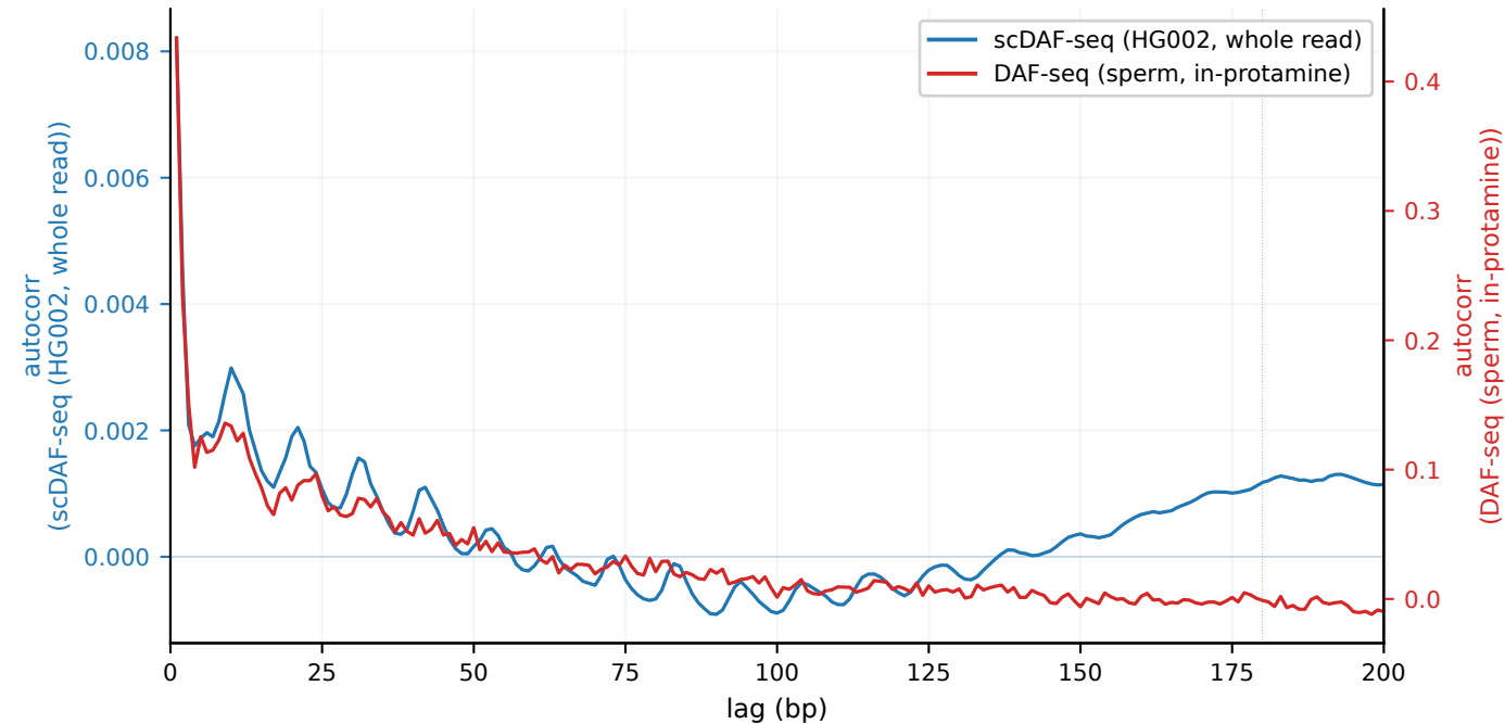
A · DAF-based deamination periodicity
