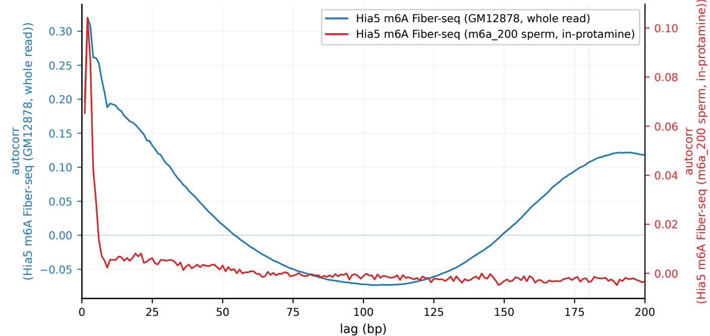
B · Hia5 m6A periodicity
