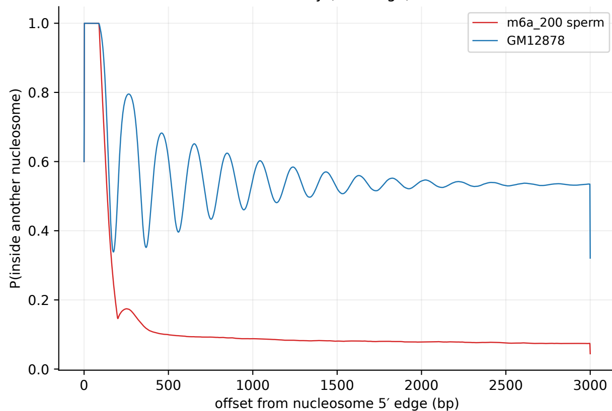
A. Downstream nucleosome density (full range)
