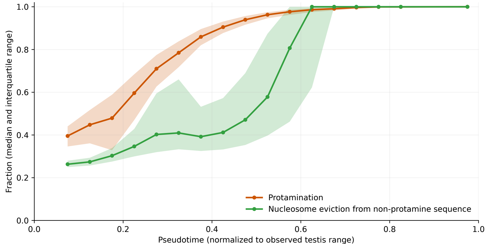
Chromatin transition trajectory
