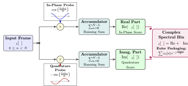
Figure 1.3a: Probe-wave quadrature interferometer. (1) What it is: Internal architecture of a single Fourier frequency bin evaluated as a dual-branch correlation receiver. (2) What to look at: Incoming frame \ell[n] splits into branches multiplied by \cos(2\pi f_k n / N) (in-phase) and -\sin(2\pi f_k n / N) (quadrature), accumulating into real and imaginary coordinates. (3) What it proves: Complex numbers represent the two orthogonal axes needed to measure wave energy independently of arrival phase.
