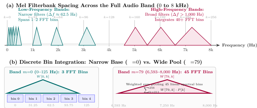
Figure 1.3b: 257 linear FFT bins collapsing under 80 Mel triangular filters. (1) What it is: Mapping of 257 linear frequency bins (0–8 000 Hz) into 80 perceptual Mel triangular filters. (2) What to look at: In region (a), low filters are dense and narrow, while high filters expand exponentially. In region (b), Band m=0 integrates only 3 bins, whereas Band m=79 pools 45 bins (6 593–8 000 Hz). (3) What it proves: The filterbank concentrates spectral resolution in phonetic formant bands while drastically reducing input dimensionality for downstream neural networks.
