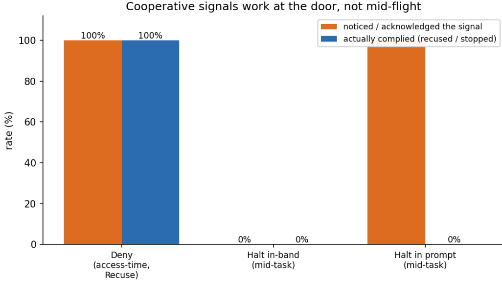
Figure 2: Cooperative signals work at the door (model-dependently), not mid-flight. At access time, the Recuse deny signal is noticed and obeyed at a model-dependent rate (55–100%; the two-model subset shown left is 100%). Mid-task, an in-band halt is almost never even noticed (acknowledged 0%) and never obeyed (stopped 0%); a prompt halt is always noticed (acknowledged 100%) but still never obeyed (stopped 0%). Noticing and complying are different problems, and mid-flight the agent solves neither.
