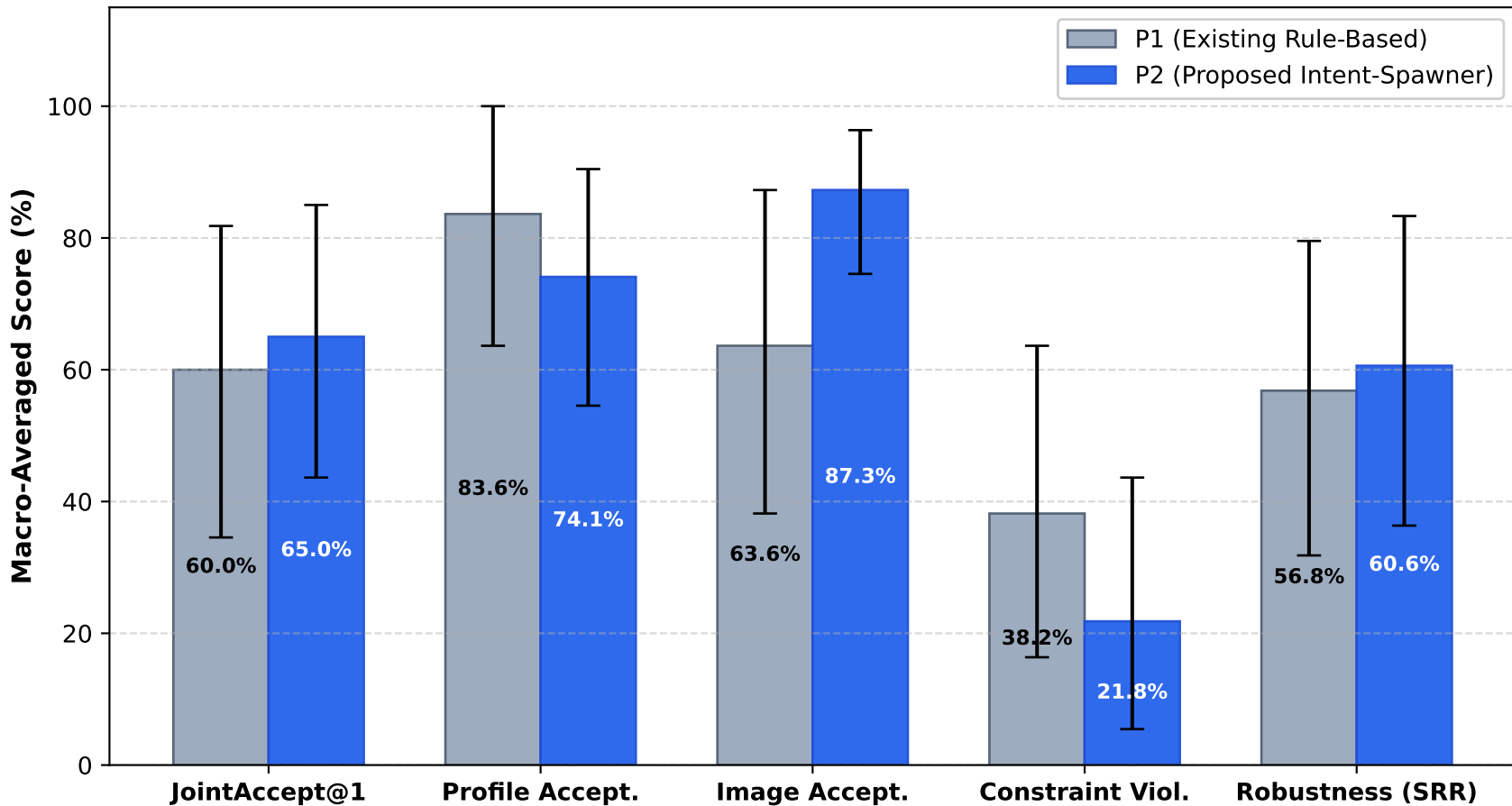
E1 Recommendation Quality and Robustness (Macro-Average with 95% Bootstrap CI)
