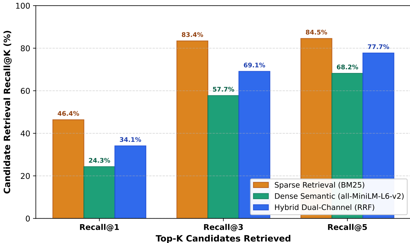
Candidate Retrieval Channel Ablation Across Recall@K
