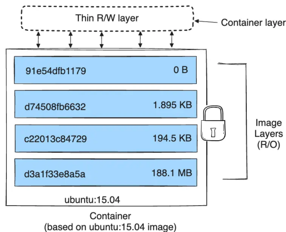
Figure 2.3. Layered container image architecture with stacked read-only layers and a top read-write container layer [6]
