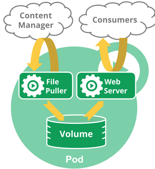
Figure 2.2. Conceptual structure of a Kubernetes Pod encapsulating containers and shared storage volumes [22]
