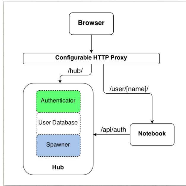
Figure 2.1. Subsystem architecture of JupyterHub showing the Hub, Configurable HTTP Proxy, Spawner, and single-user notebook servers [15]
