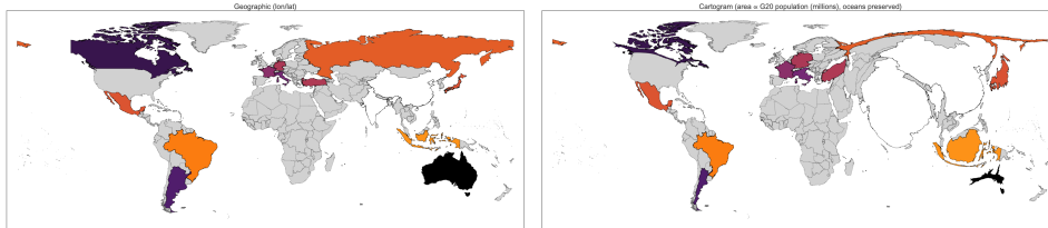
Figure 3. A cartogram driven by a hand-curated Association of 19 G20-ish economies; every other country appears in grey and does not contribute to the density field, but still visibly deforms because diffusion is global.
